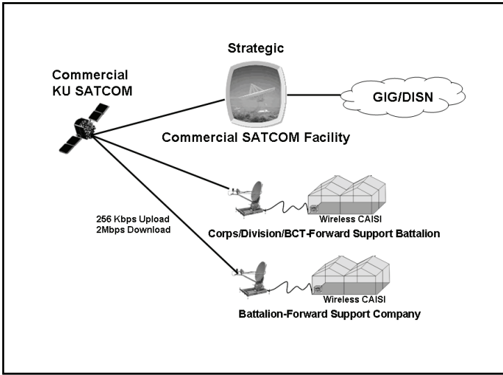
Figure 6-1. CSS VSAT architecture
